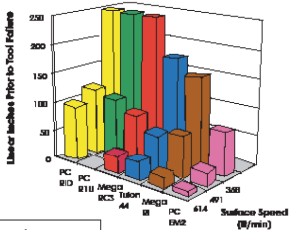
Figure #1 Ultimate Tool Life as a Function of Surface Speed
